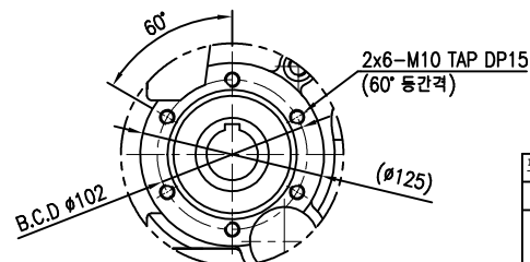
OUTPUT MOUNTING
