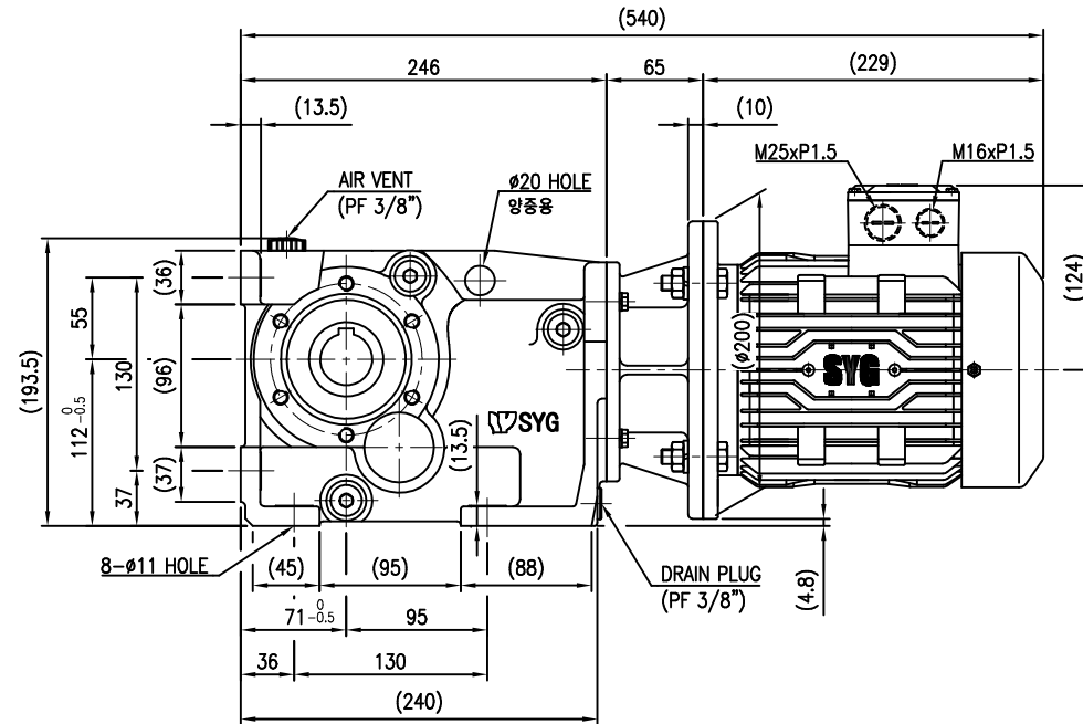
60° 2x6-M10 TAP DP15 (60° 등간격) (Ø125) B.C.D Ø102
