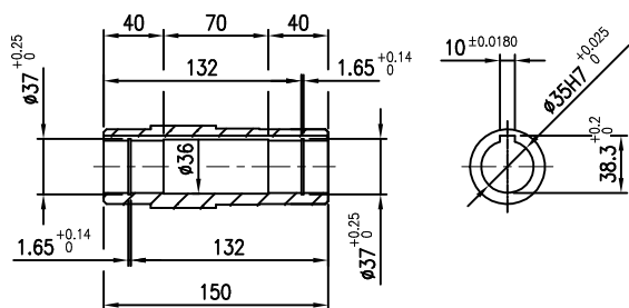
OUTPUT SHAFT(HOLLOW)
