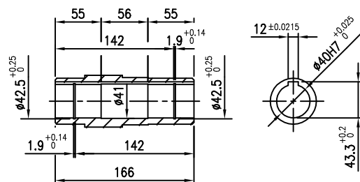
OUTPUT SHAFT(HOLLOW)
