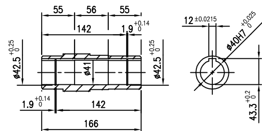
OUTPUT SHAFT(HOLLOW)
