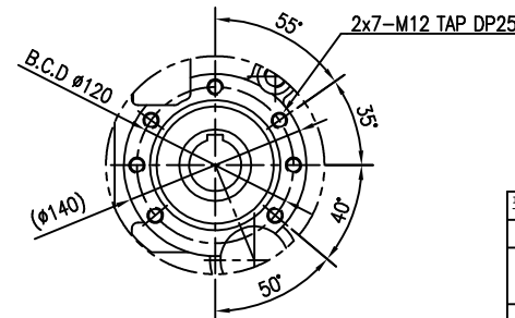
OUTPUT MOUNTING
