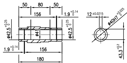
OUTPUT SHAFT(HOLLOW)
