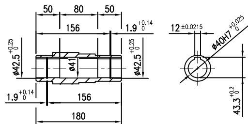
OUTPUT SHAFT(HOLLOW)
