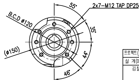
OUTPUT MOUNTING
