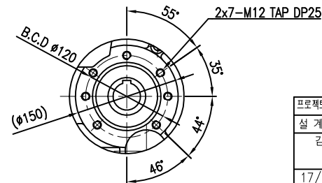
OUTPUT MOUNTING
