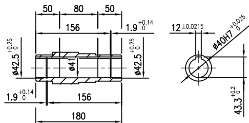
OUTPUT SHAFT(HOLLOW)
