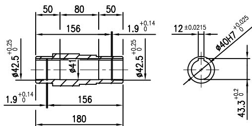
OUTPUT SHAFT(HOLLOW)
