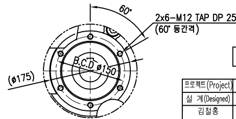
OUTPUT MOUNTING
