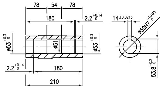
OUTPUT SHAFT(HOLLOW)
