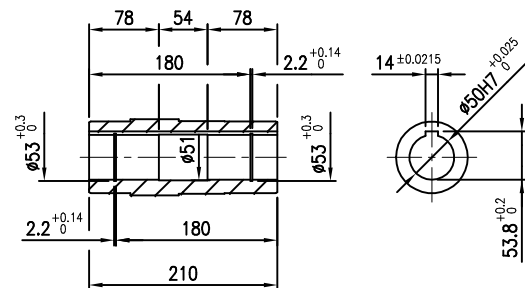
OUTPUT SHAFT(HOLLOW)
