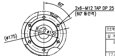
OUTPUT MOUNTING
