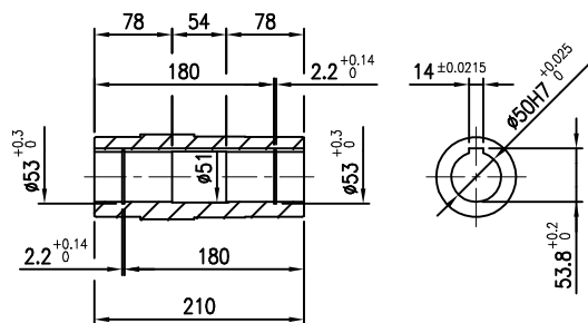
OUTPUT SHAFT(HOLLOW)
