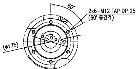
OUTPUT MOUNTING
