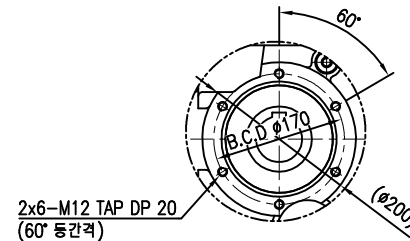
OUTPUT MOUNTING
