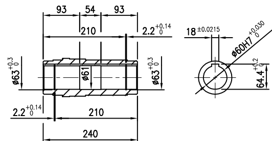
OUTPUT SHAFT(HOLLOW)
