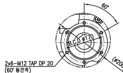
OUTPUT MOUNTING
