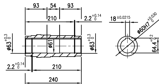
OUTPUT SHAFT(HOLLOW)
