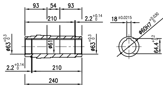
OUTPUT SHAFT(HOLLOW)
