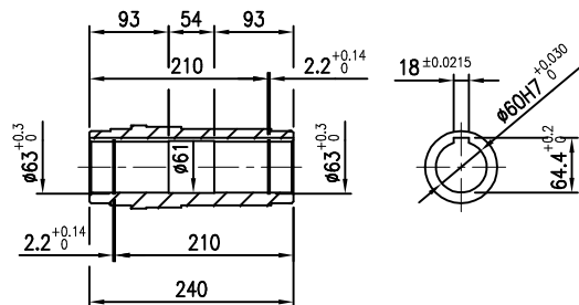
OUTPUT SHAFT(HOLLOW)
