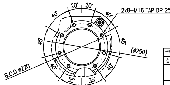
OUTPUT MOUNTING
