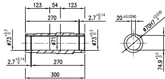
OUTPUT SHAFT(HOLLOW)
