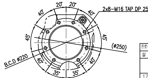
OUTPUT MOUNTING
