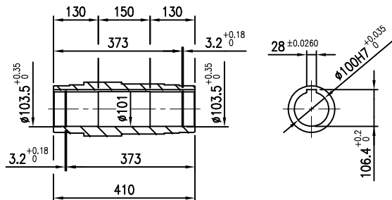
OUTPUT SHAFT(HOLLOW)
