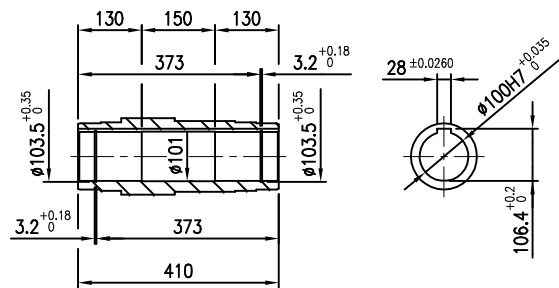
OUTPUT SHAFT(HOLLOW)
