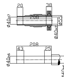
Shrink disk
