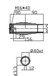
Hollow shaft
