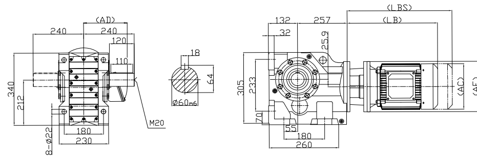
DK87
