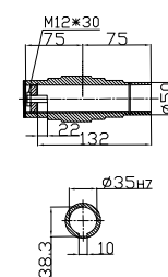
Hollow shaft
