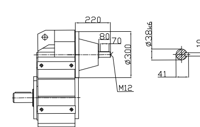
DF..S97
