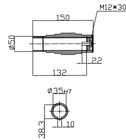
Hollow shaft
