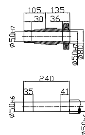
Shrink disk
