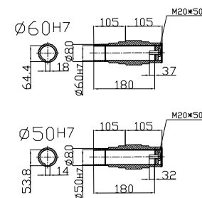
Hollow shaft
