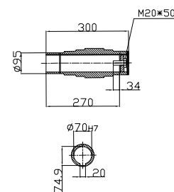
Hollow shaft
