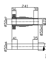
Shrink disk
