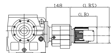
DS..77DR37
