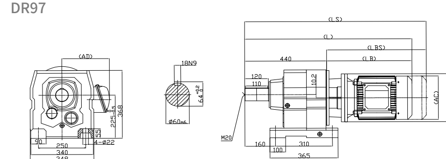
DR97
