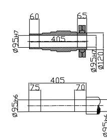
Shrink disk
