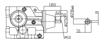
DK..S87
