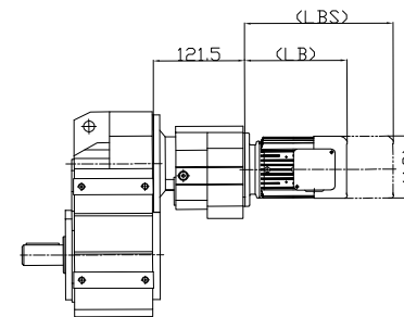
DF..47DR17
