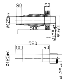
Shrink disk
