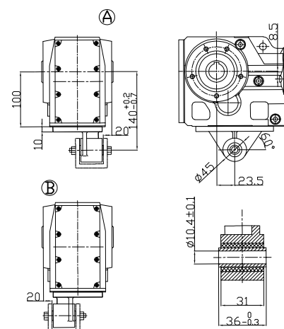
Hollow shaft
