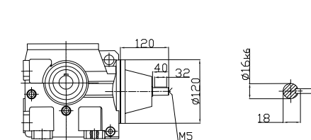
DS..S57
