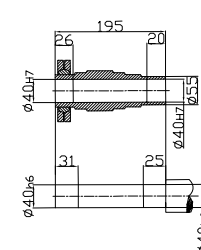
Shrink disk
