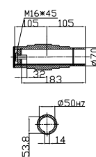
Hollow shaft
