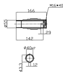
Hollow shaft
