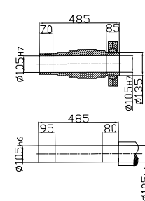
Shrink disk
