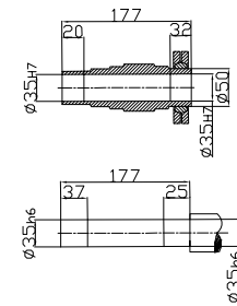
Shrink disk
