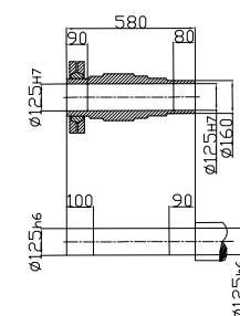
Shrink disk
