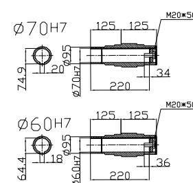
Hollow shaft
