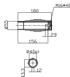
Hollow shaft
