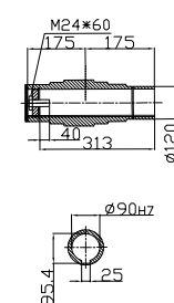
Hollow shaft
