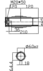
Hollow shaft
