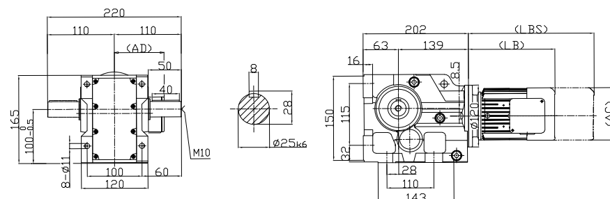
DKAT37
