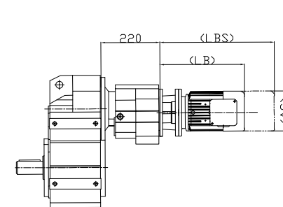
DF..107DR77
