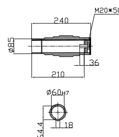
Hollow shaft
