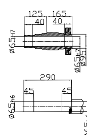
Shrink disk
