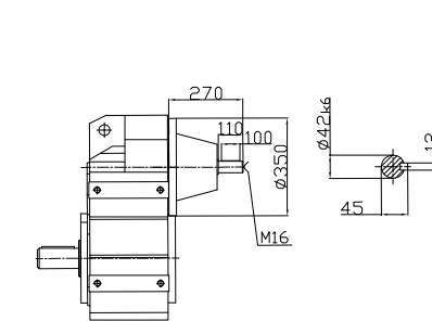
DF..S107
