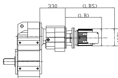
DF..157DR97
