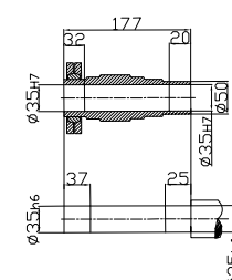
Shrink disk
