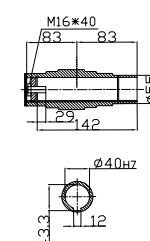
Hollow shaft
