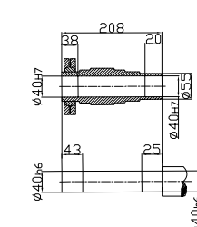
Shrink disk
