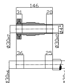
Shrink disk
