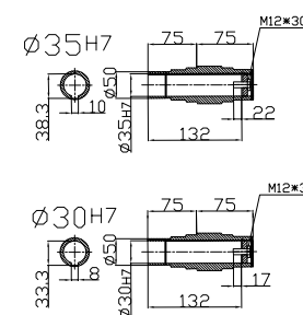
Hollow shaft
