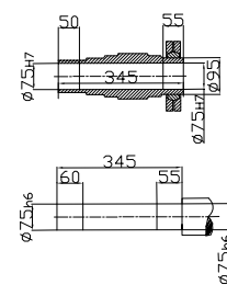
Shrink disk
