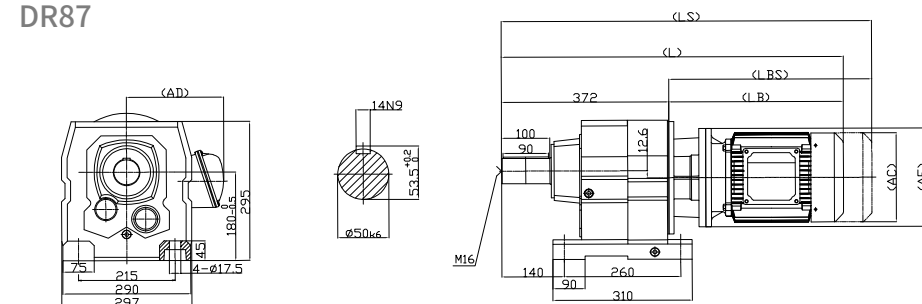
DR87
