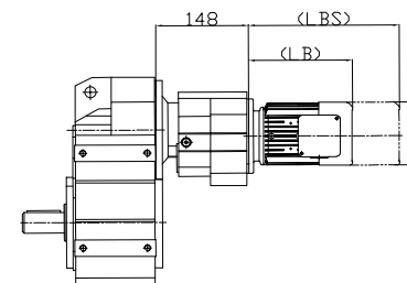
DF..77DR37
