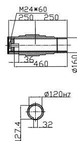
Hollow shaft
