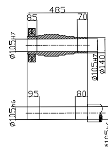
Shrink disk
