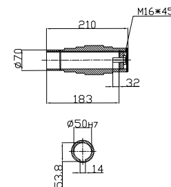
Hollow shaft
