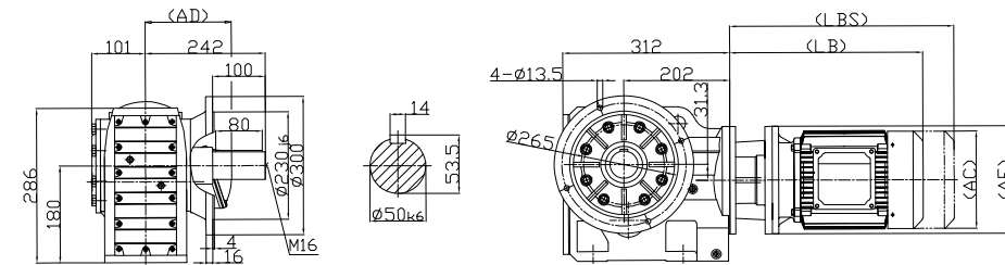
DKF77
