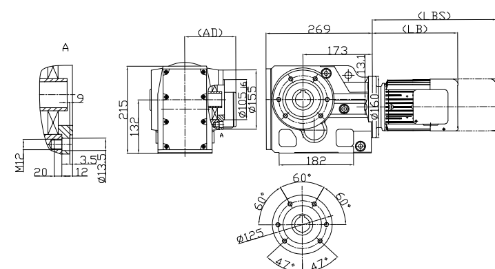
DKAZ57
