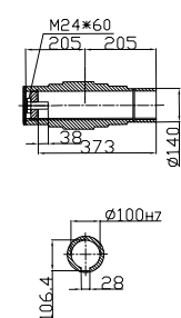
Hollow shaft
