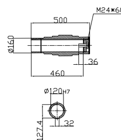
Hollow shaft
