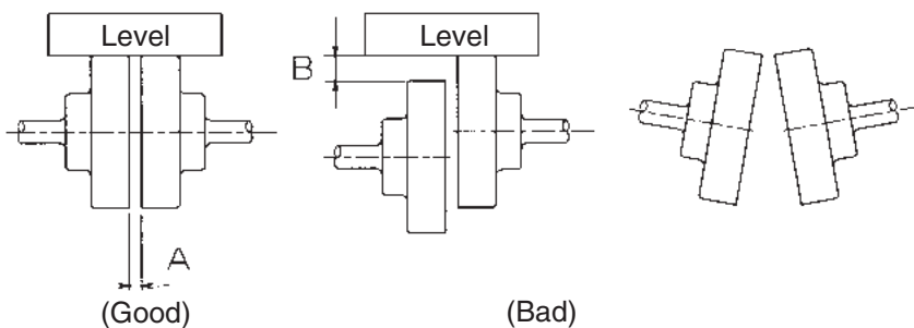
Fig. 12 Installation of coupling
