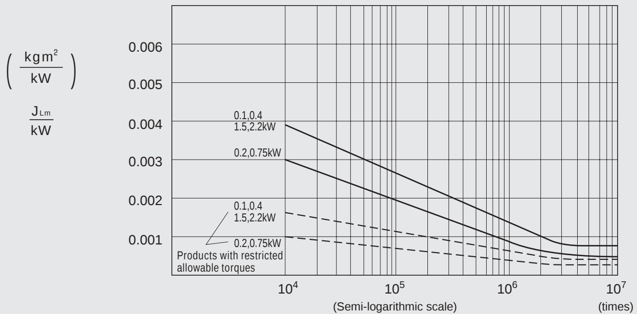
Fig. 11 GM-SHY/SHYP Series
