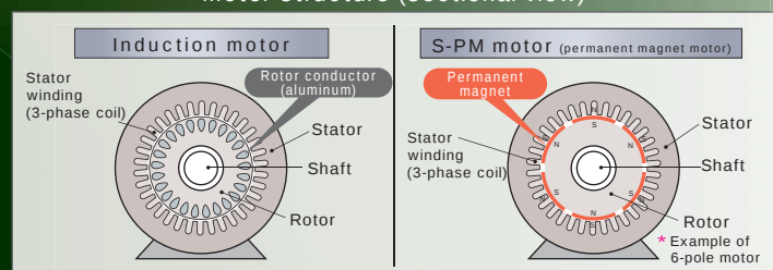
Motor structure (sectional view)
