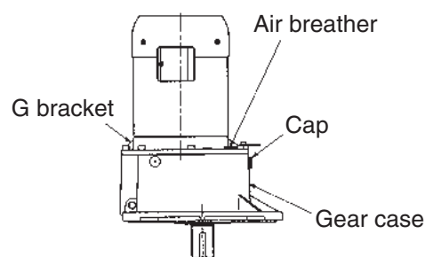
In the case of vertical installation
