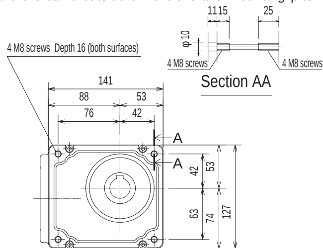
<Face mounting>
