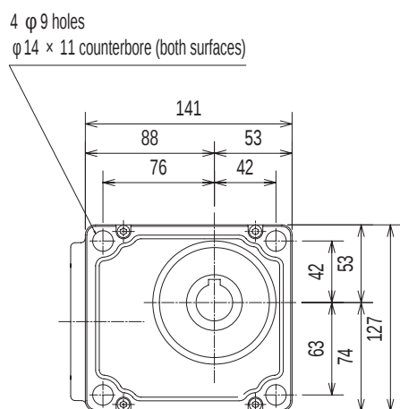
<Flange mounting>
