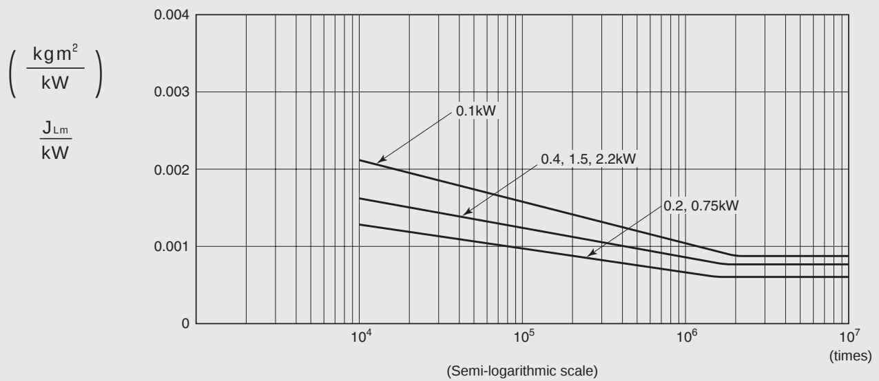
Fig. 10 GM-SSY/SSYP Series
