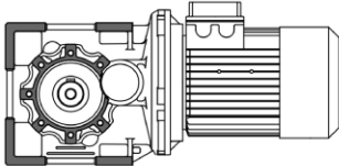
P FOOT MOUNTING / P DOUBLE OUTPUT SHAFT
