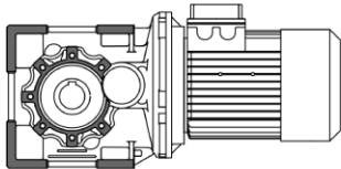
C FOOT MOUNTING / C HOLLOW SHAFT
